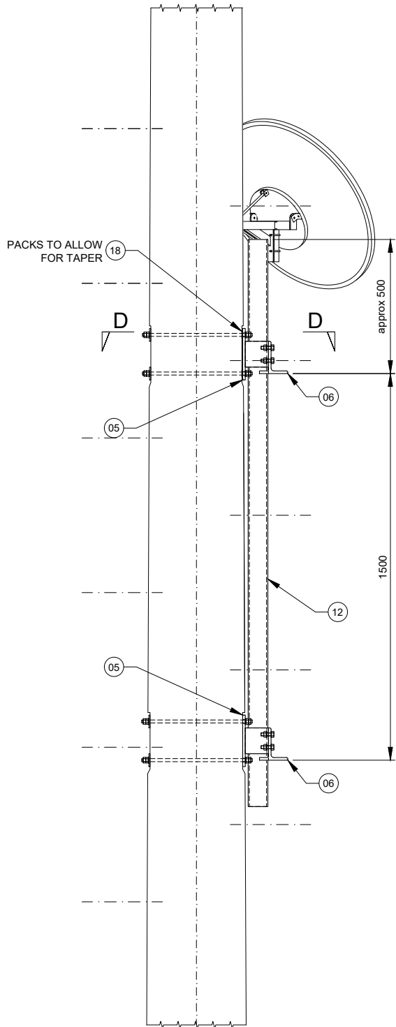
DETAIL H - VSAT DISH MOUNT Scale 1:20
