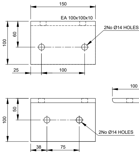
TPL-A - EA100x100x10 Scale 1:5
