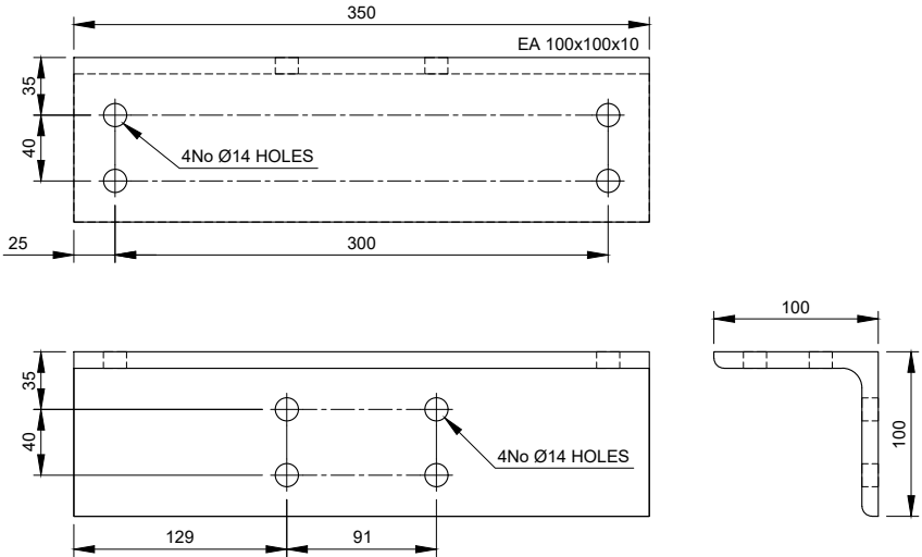
TPY-A - EA100x100x10 Scale 1:5
